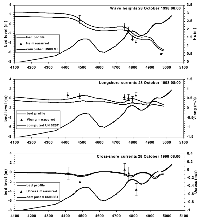
Figure 2 Comparison of cross-shore distributions of wave height, longshore velocity and cross-shore velocity for Event 1 (28-10-1998 9:00).
