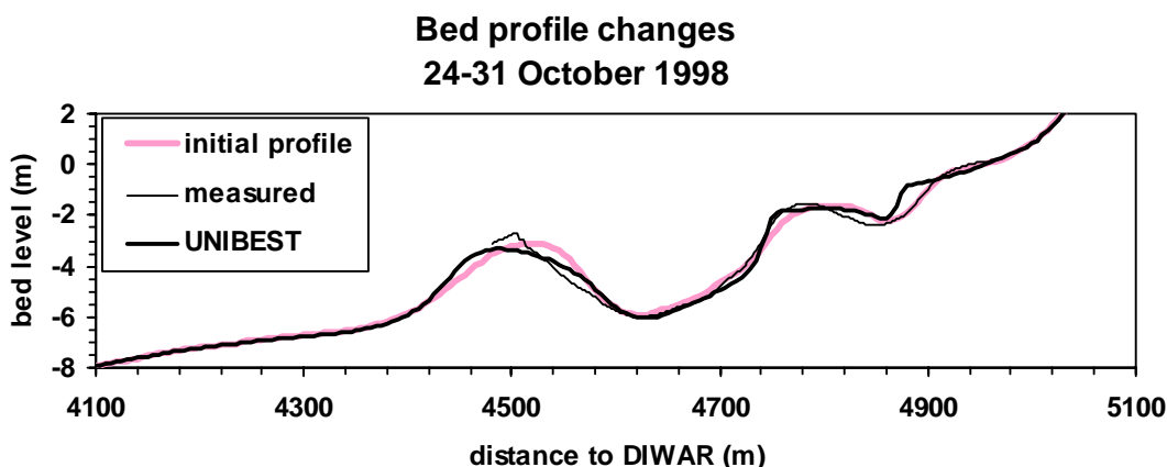
Figure 5 Comparison of profile predictions during major storm period 24-31 Oct.
