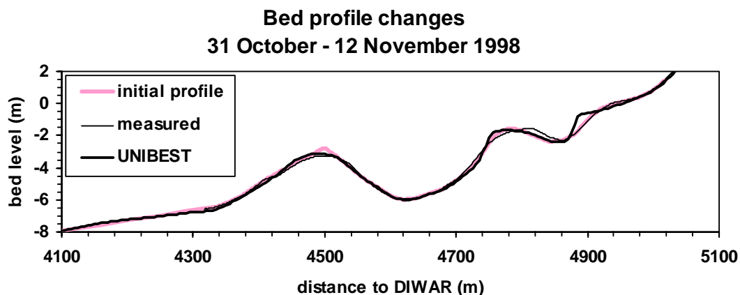
Figure 6 Comparison of profile predictions during minor storm period 31 Oct - 12 Nov.
