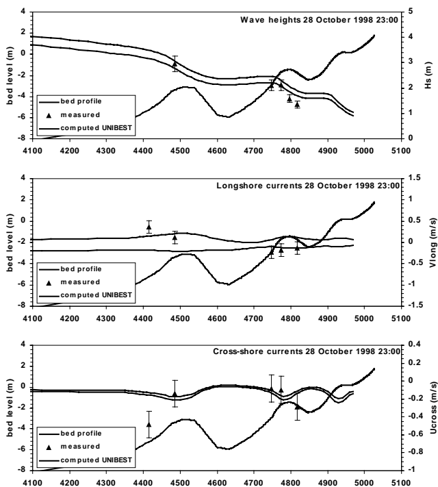
Figure 4 Comparison of cross-shore distributions of wave height, longshore velocity and cross-shore velocity for Event 3 (28-10-1998 23:00).
