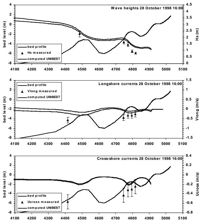
Figure 3 Comparison of cross-shore distributions of wave height, longshore velocity and cross-shore velocity for Event 2 (28-10-1998 16:00).
